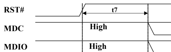
Figure 18. MDC/MDIO Reset Timing
