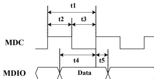
Figure 16. MDC/MDIO Write Timing
