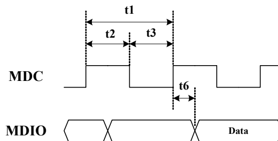
Figure 17. MDC/MDIO Read Timing
