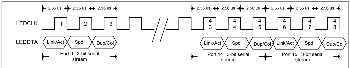
Figure 13. 3-Bit Serial Stream Mode
