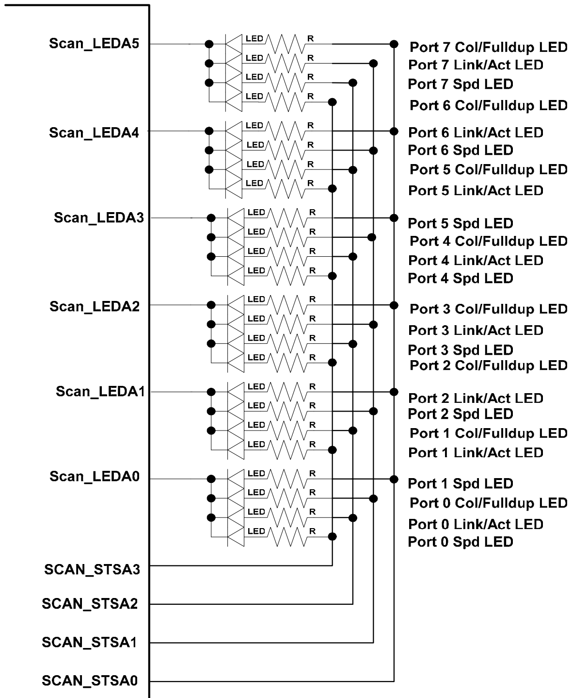
Figure 15. External Circuit for Scan LED
